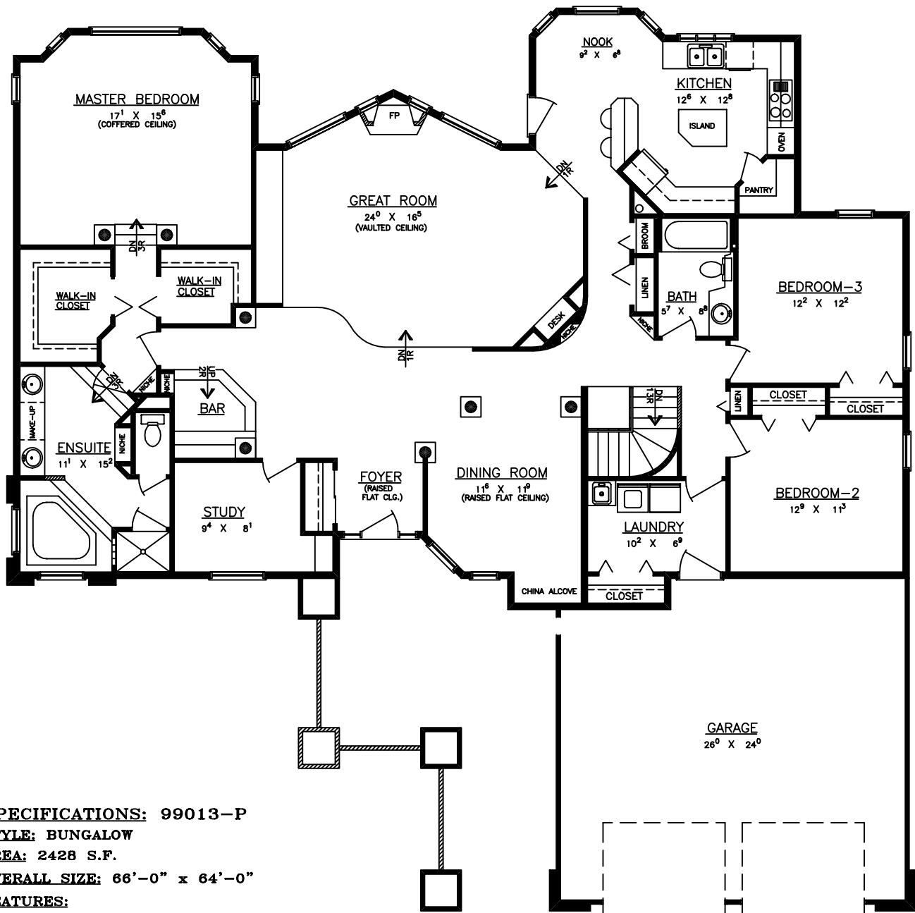
FLOOR PLAN
